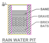
RAIN WATER PIT
