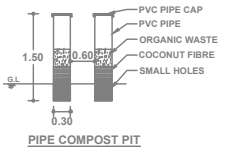
PIPE COMPOST PIT
