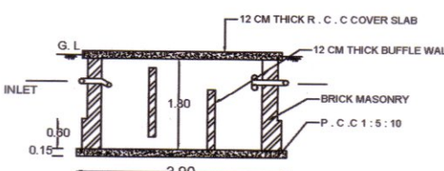
SECTION ON B-B
