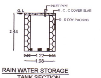
RAIN WATER STORAGE TANK SECTION
