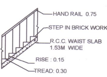
STAIR CASE SECTION
