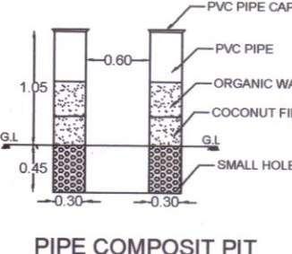
PIPE COMPOSIT PIT
