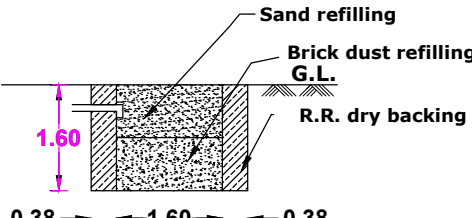
DETAILS OF RAIN WATER HARVESTING Dwg:1A
