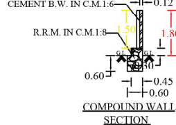
COMPOUND WALL SECTION
