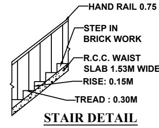
STAIR DETAIL
