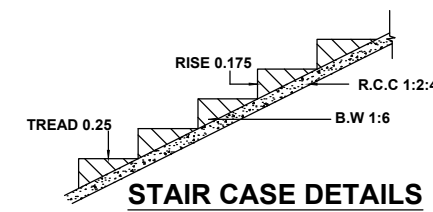
STAIR CASE DETAILS
