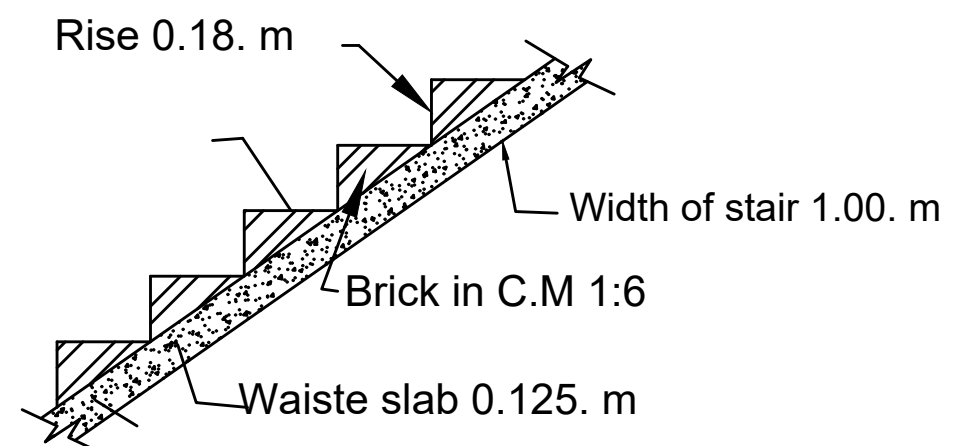
Stair Details
