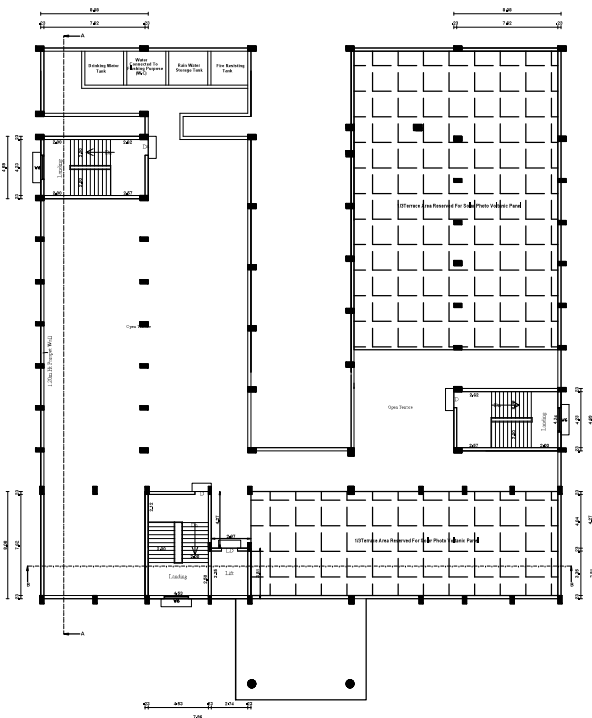
TERRACE FLOOR PLAN COLLEGE MAIN BLOCK
