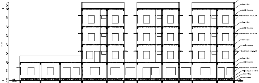
SECTION ON 'AA' DOCTORS QUARTERS
