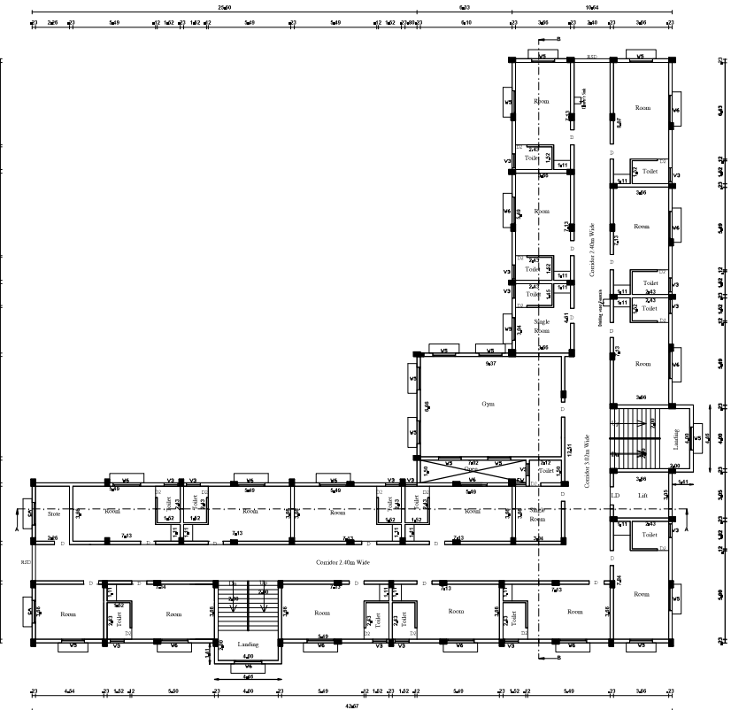
THIRD FLOOR PLAN GIRLS HOSTEL
