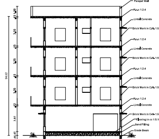
SECTION ON 'BB' DOCTORS QUARTERS
