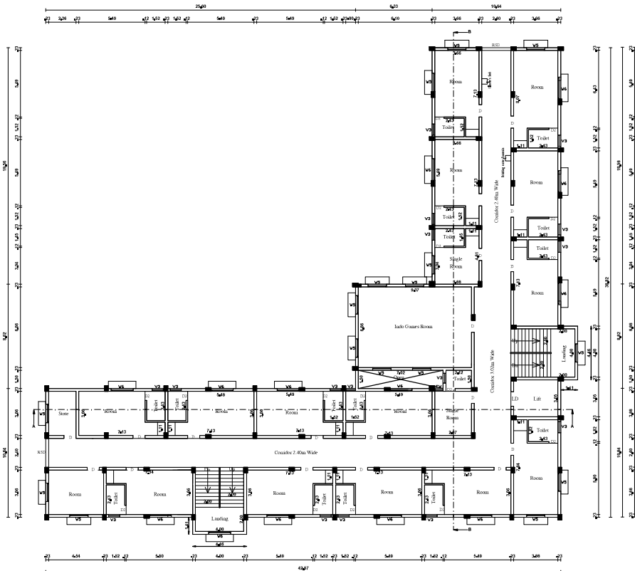
SECOND FLOOR PLAN GIRLS HOSTEL
