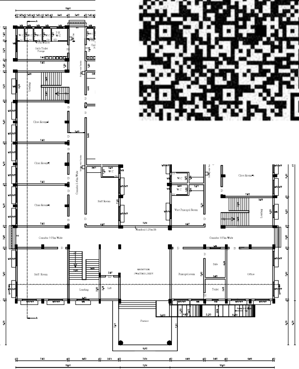
GROUND FLOOR PLAN COLLEGE MAIN BLOCK
