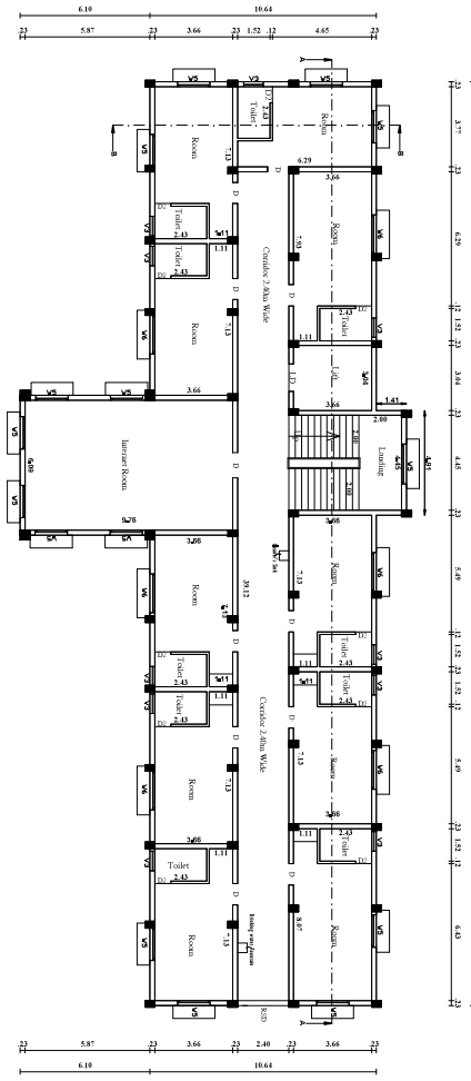
FOURTH FLOOR PLAN BOM NOTES
