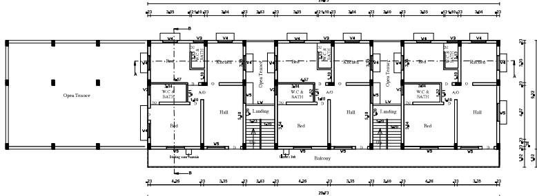
FIRST FLOOR PLAN DOCTORS QUARTERS
