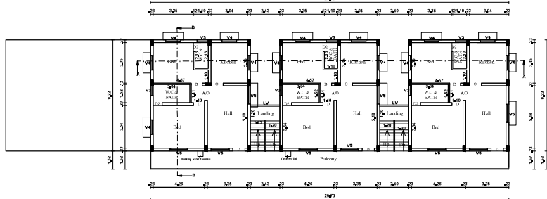
SECOND FLOOR PLAN DOCTORS QUARTERS
