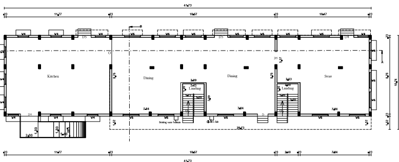
GROUND FLOOR PLAN DOCTORS QUARTERS
