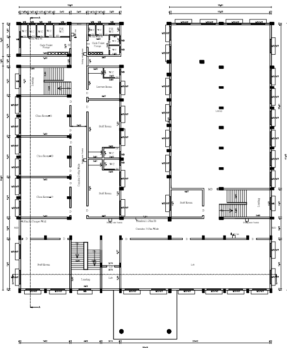
THIRD FLOOR PLAN COLLEGE MAIN BLOCK
