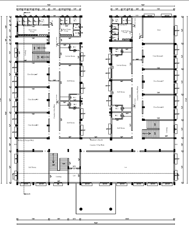
SECOND FLOOR PLAN COLLEGE MAIN BLOCK
