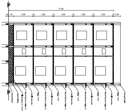
SECTION ON 'BB' BOYS HOSTEL
