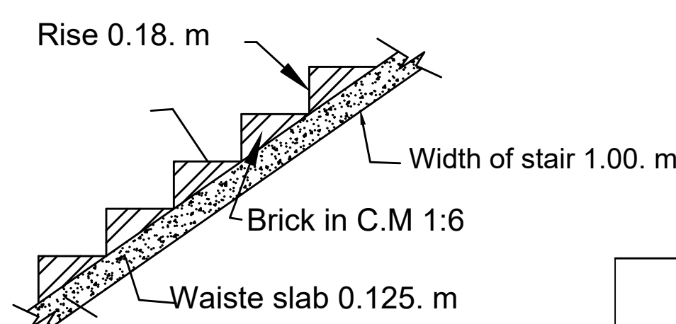
Stair Details
