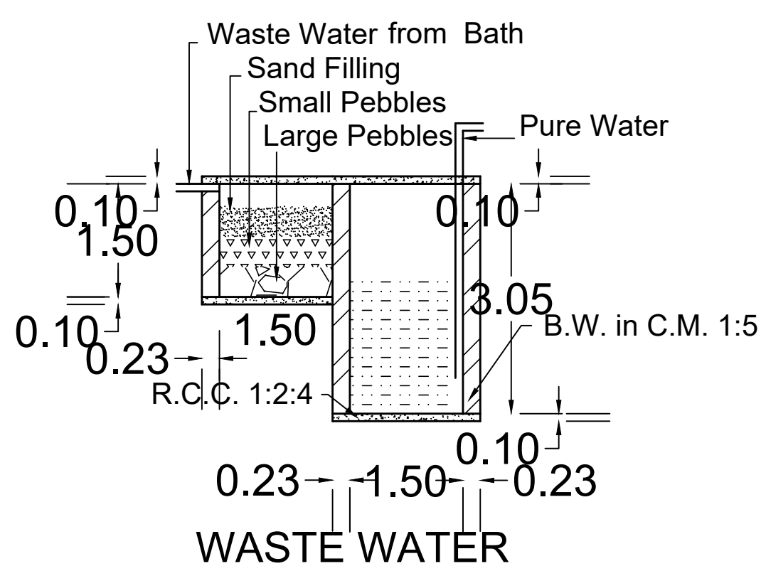
RECYCLING SYSTEM
