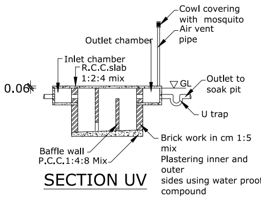
RECYCLING OF WASTE WATER SYSTEM
