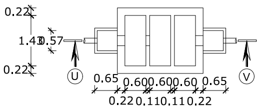
SECTION UV
