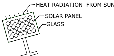
SOLAR SYSTEM
