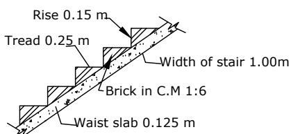
STAIR DETAILS
