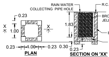
RAIN WATER HARVEST WELL
