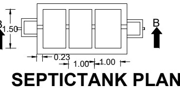
SEPTICTANK PLAN
