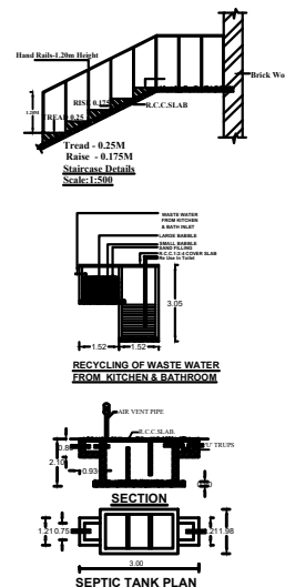
SEPTIC TANK PLAN
