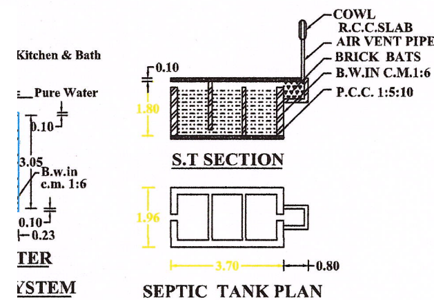
SEPTIC TANK PLAN
