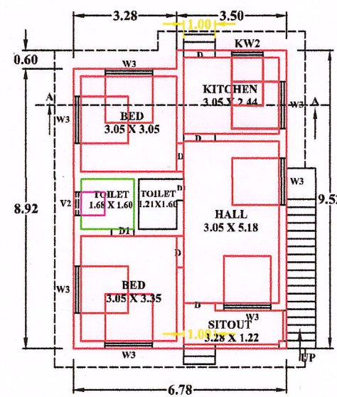
PLAN(GROUND FLOOR)
