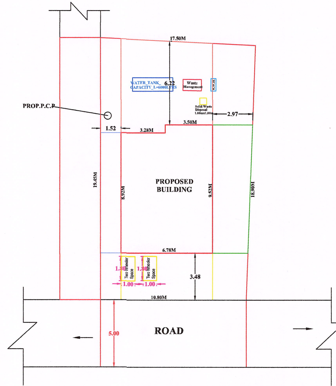
SITE PLAN
