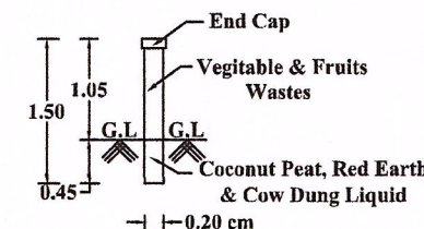
PIPE COMPOSTER
