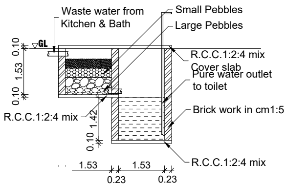
WATER RECYCLING SYSTEM
