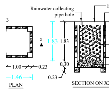
WATER HARVEST WELL
