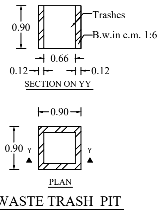
WASTE TRASH PIT
