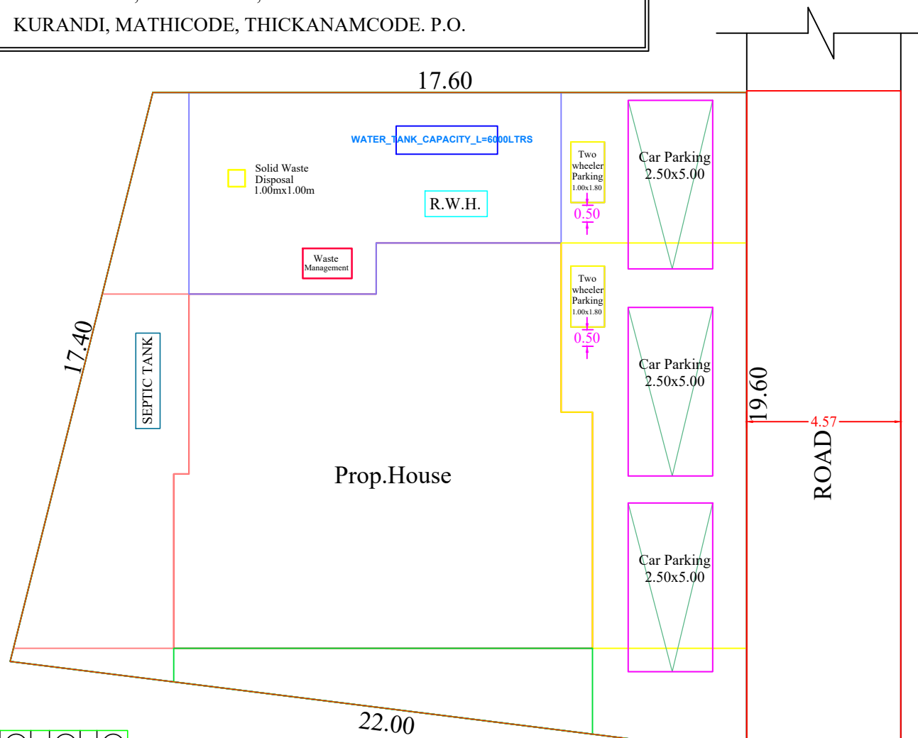
SITE PLAN
