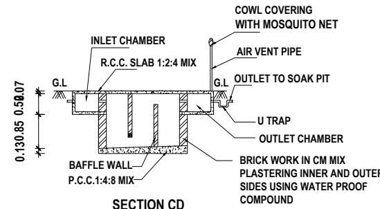
SECTION CD
