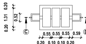
SECTION CD
