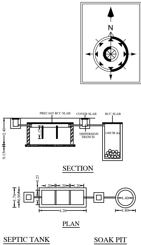
SEPTIC TANK SOAK PIT
