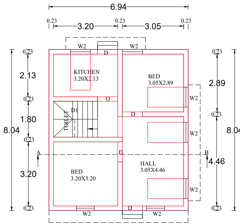
LOOR PLAN
