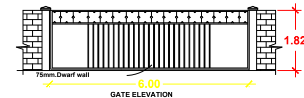
GATE ELEVATION
