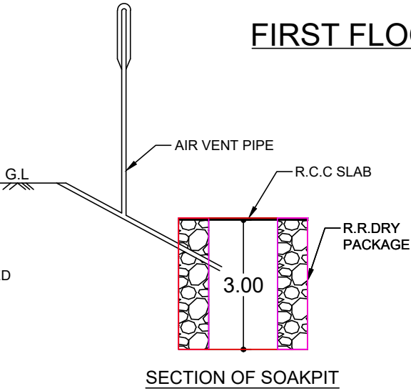
SECTION OF SOAKPIT
