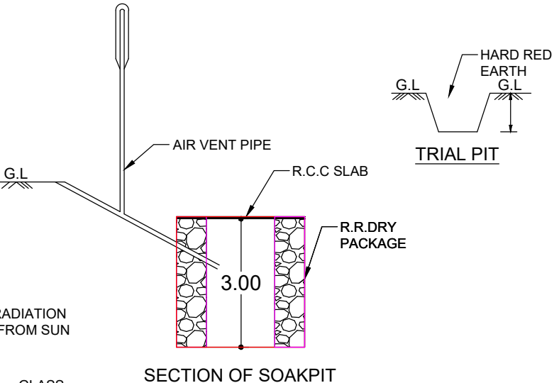
SECTION OF SOAKPIT
