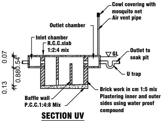
SECTION UV
