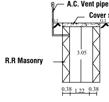
Soakpit section
