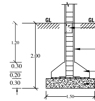
SECTION OF COLUMN
