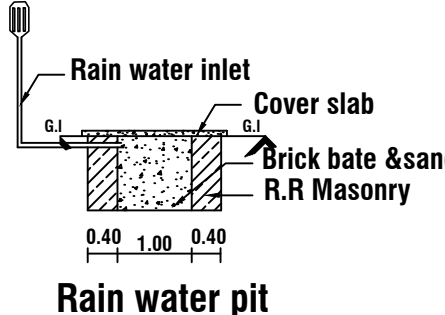
Rain water pit
