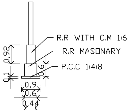
FOUNDATION
