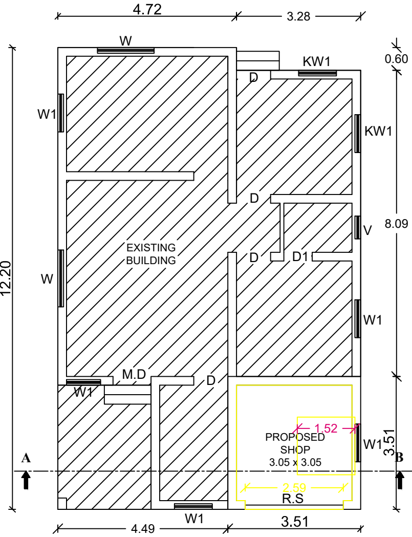
EXISTING GROUND FLOOR (D.NO:8-243) & PROPOSED SHOP PLAN
