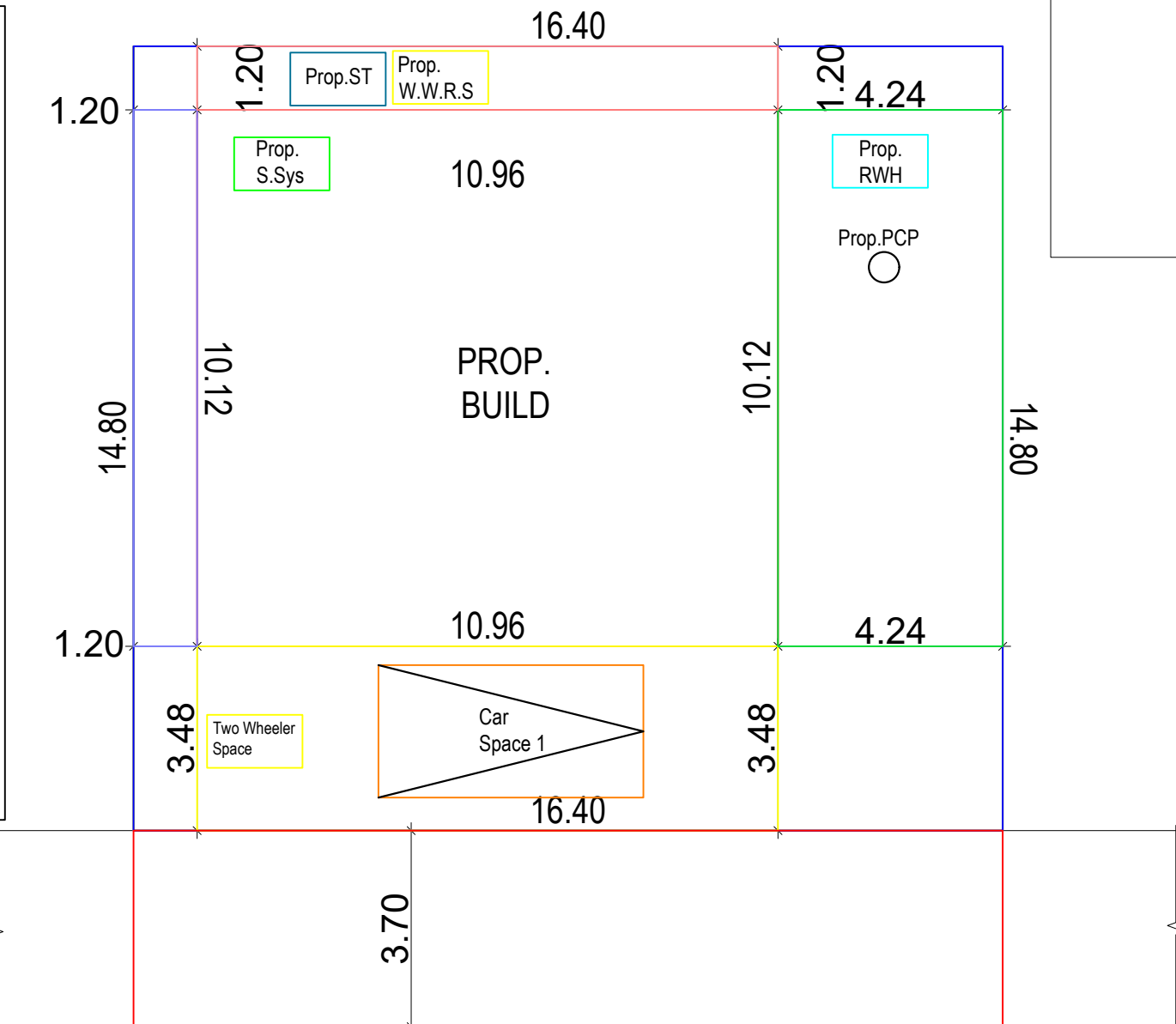
SITE PLAN
