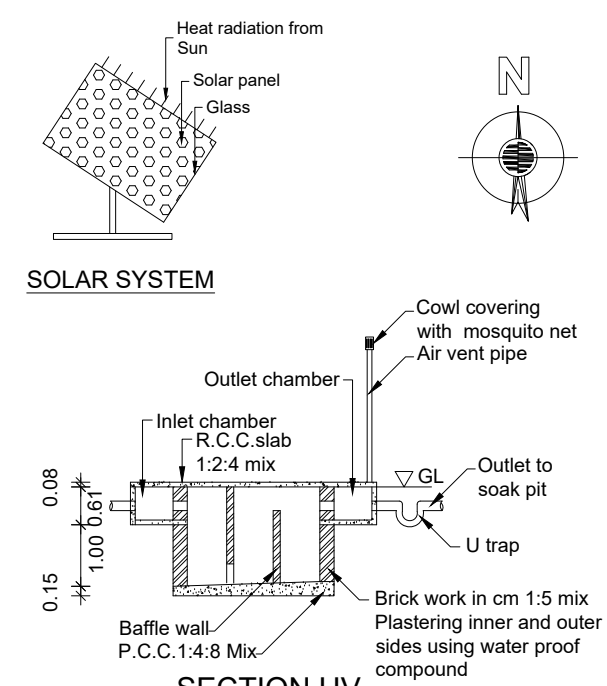
SECTION UV
