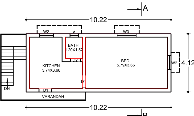
FIRST FLOOR PLAN (RESIDENTIAL)
