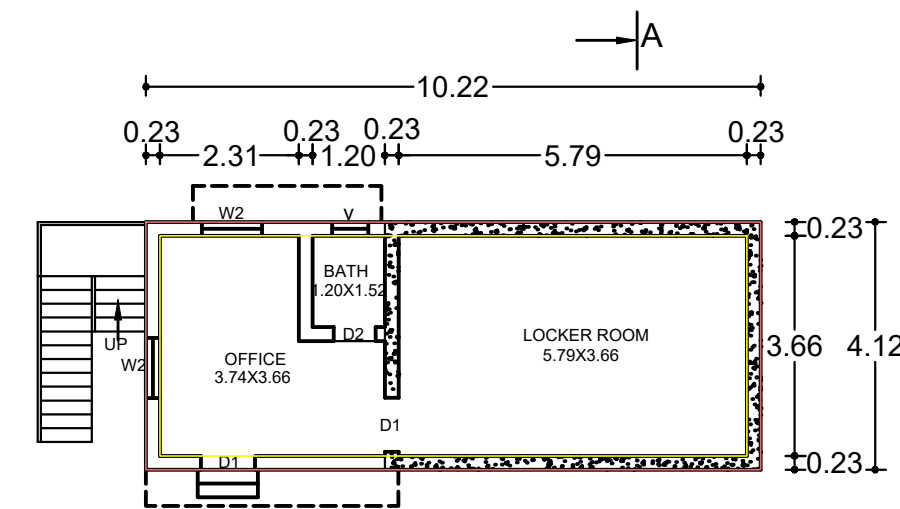
GROUND FLOOR PLAN (COMMERCIAL)
