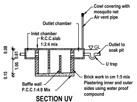
SECTION UV
