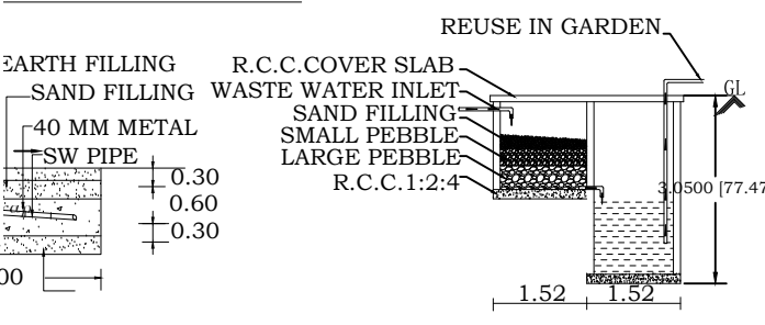
SECTION OF DISPERSION TRENCH
