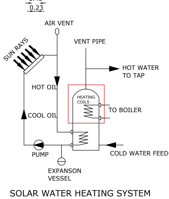
SOLAR WATER HEATING SYSTEM
