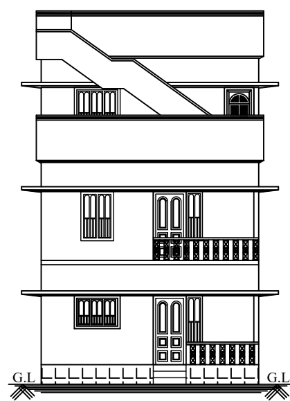
FRONT ELEVATION
