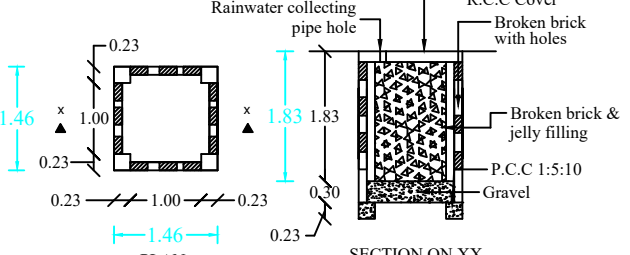
RAIN WATER HARVEST WELL RWH CAPACITY L=6642LTRS
