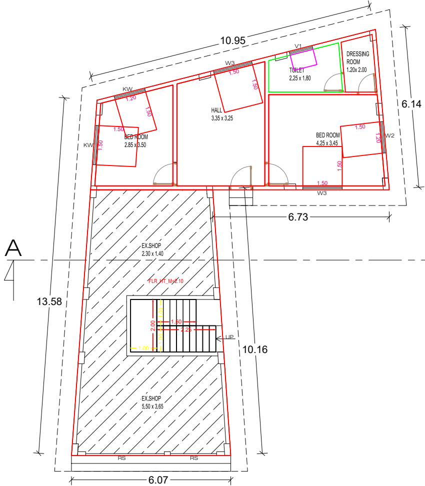
EX & ADDL. GROUND FLOOR PLAN
