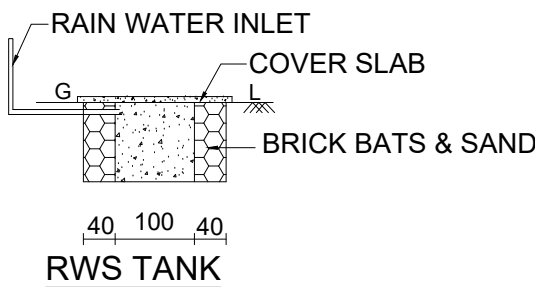
RWS TANK
