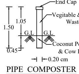
PIPE COMPOSTER
