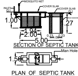
PLAN OF SEPTIC TANK
