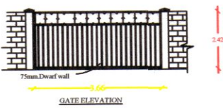
GATE ELEVATION
