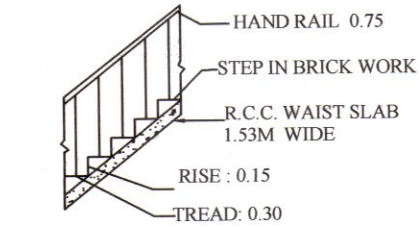
STAIR CASE SECTION
