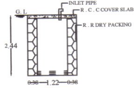
RAIN WATER STORAGE TANK SECTION
