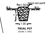
TRIAL PIT (Scale 1:100)
