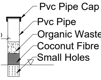
POST PIT
