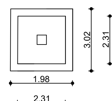
COMPOST PIT - PLAN
