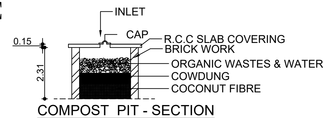
COMPOST PIT - SECTION
