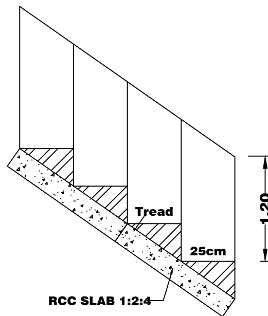
STAIR DETAILS
