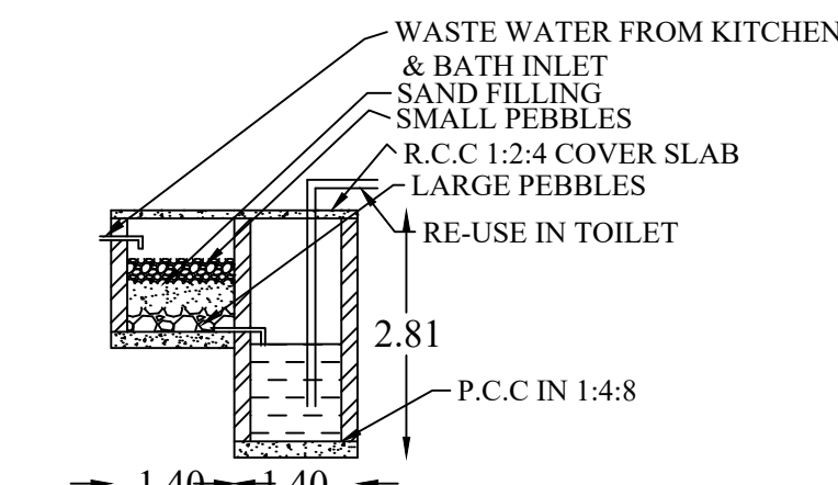
RECYCLING OF WASTE WATER KITCHEN & BATHROOM
