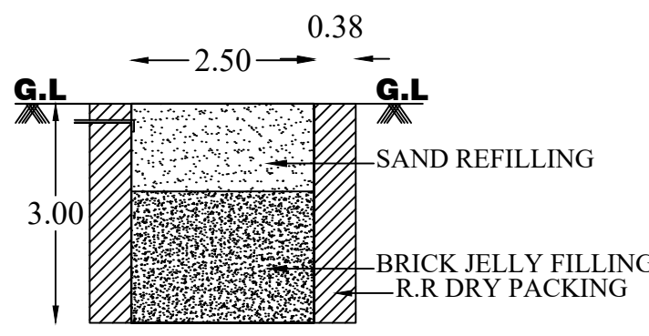
RAINWATER HARVESTING
