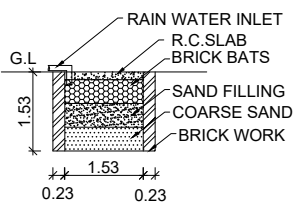
RAIN WATER HARVESTING TANK
