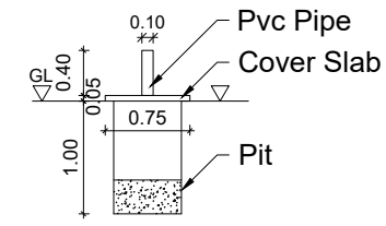
SOLID WASTE COMPOST PIT
