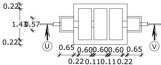
SECTION UV
