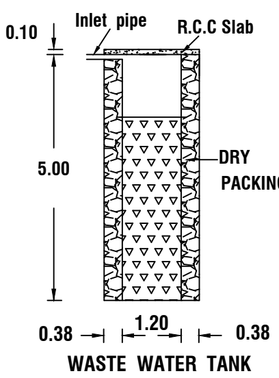
WASTE WATER TANK
