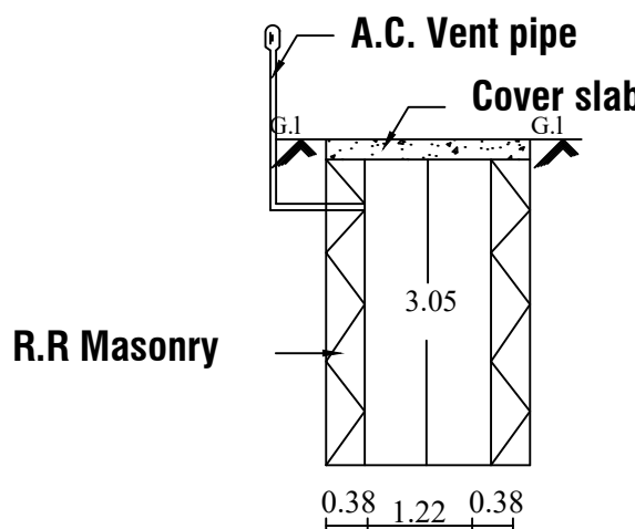
Soakpit section
