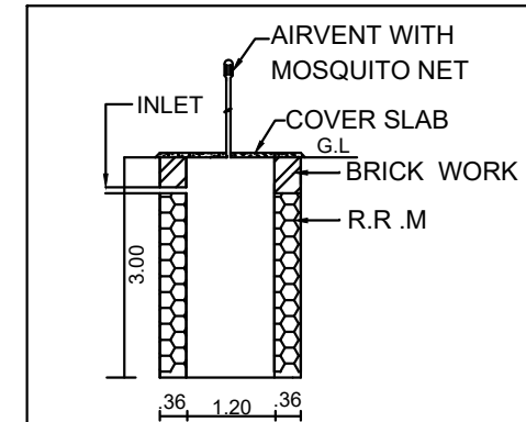
SOAK PIT - SECTION
