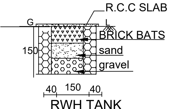
RWH TANK
