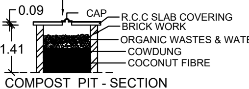
COMPOST PIT - SECTION
