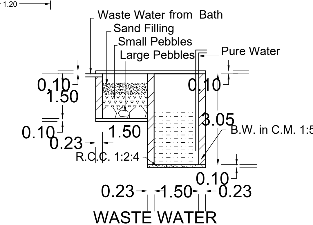
RECYCLING SYSTEM
