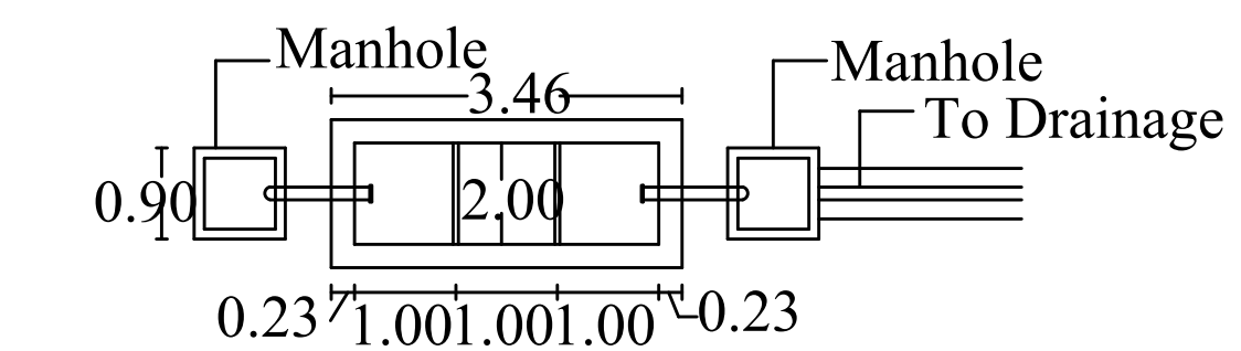
Plan Details Of Septic Tank
