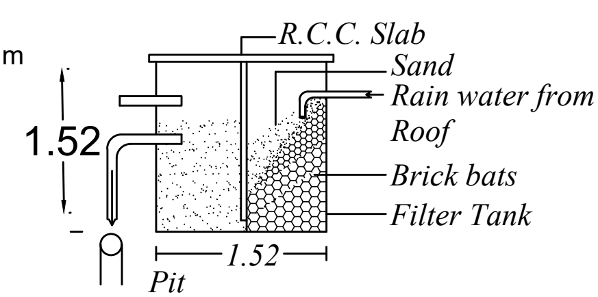
Rain Water Storage
