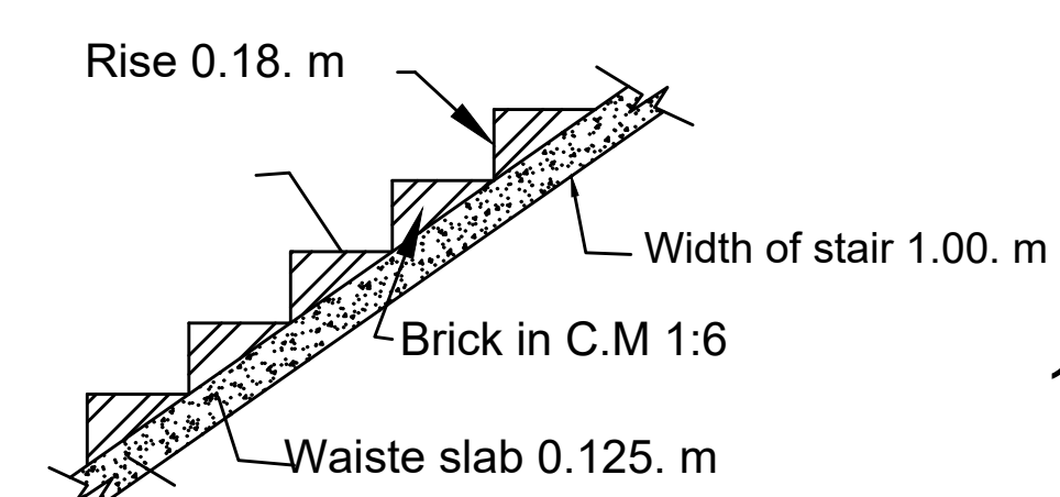
Stair Details
