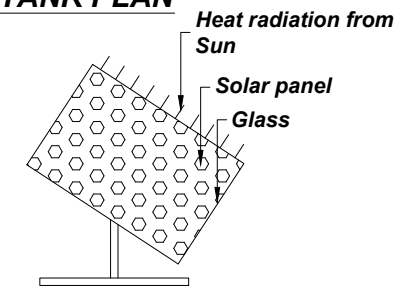
SOLAR SYSTEM
