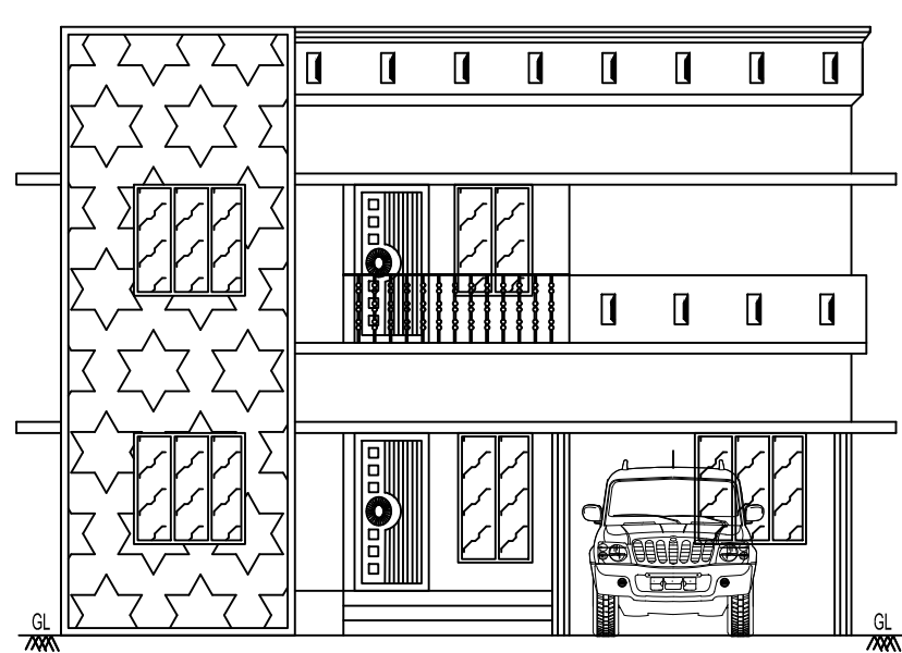
FRONT ELEVATION
