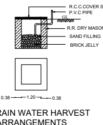
RAIN WATER HARVEST ARRANGEMENTS
