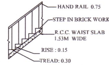
STAIR CASE SECTION
