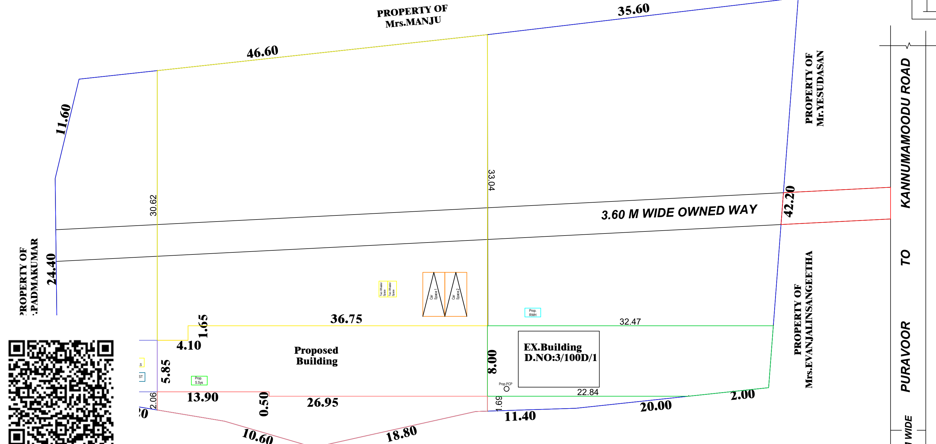
SITE PLAN SCALE 1:100 ALL DIMENSIONS ARE IN METRE
