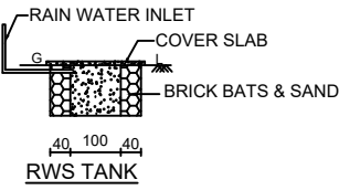
RWS TANK
