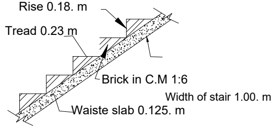
Stair Details
