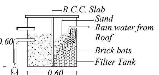
Rain Water Storage
